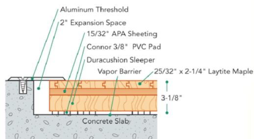
THRESHOLD DETAIL (optional accessory)
