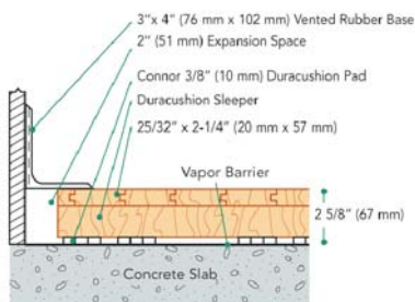
WALL BASE DETAIL
