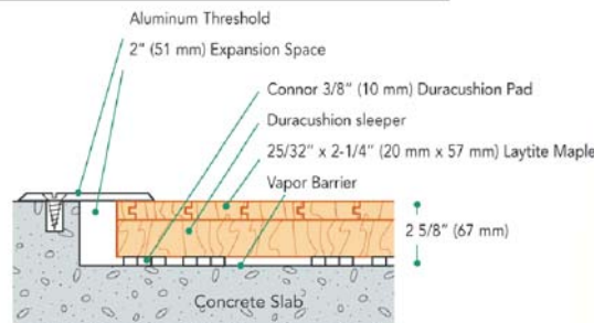
THRESHOLD DETAIL (optional accessory)
