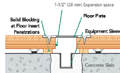
EQUIPMENT DETAIL (optional accessory)
