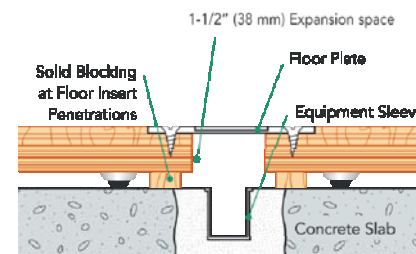
EQUIPMENT DETAIL (optional accessory)
