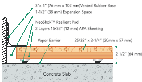
WALL BASE DETAIL
